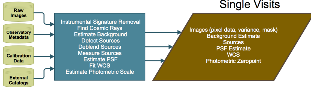
FIGURE 3: Illustration of the conceptual algorithm design for Single Visit Processing pipeline.
